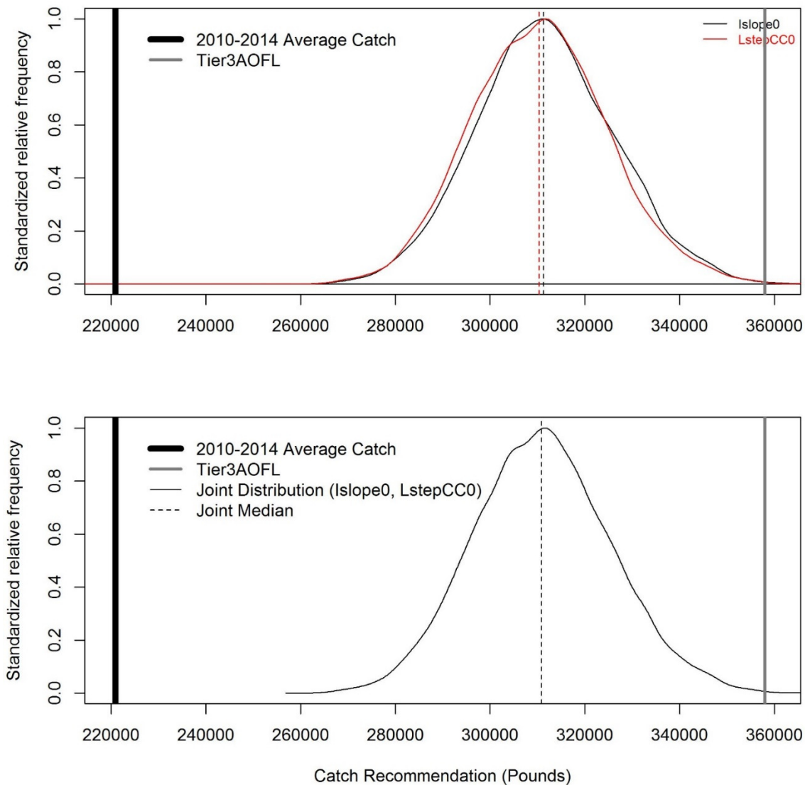
Figure 5.4 Distribution of the catch recommendation (in pounds) for Lane Snapper recommended by the two viable methods, Islope0 and LstepCC0 (top panel; dashed vertical lines identify medians) and a joint distribution assuming equal weighting (bottom panel). The average catch between 2010 and 2014 (thick black line) and the OFL specified by the Tier3AStatusQuo (thick gray line) are included for comparison. The joint distribution (bottom panel) is recommended for providing management advice.
