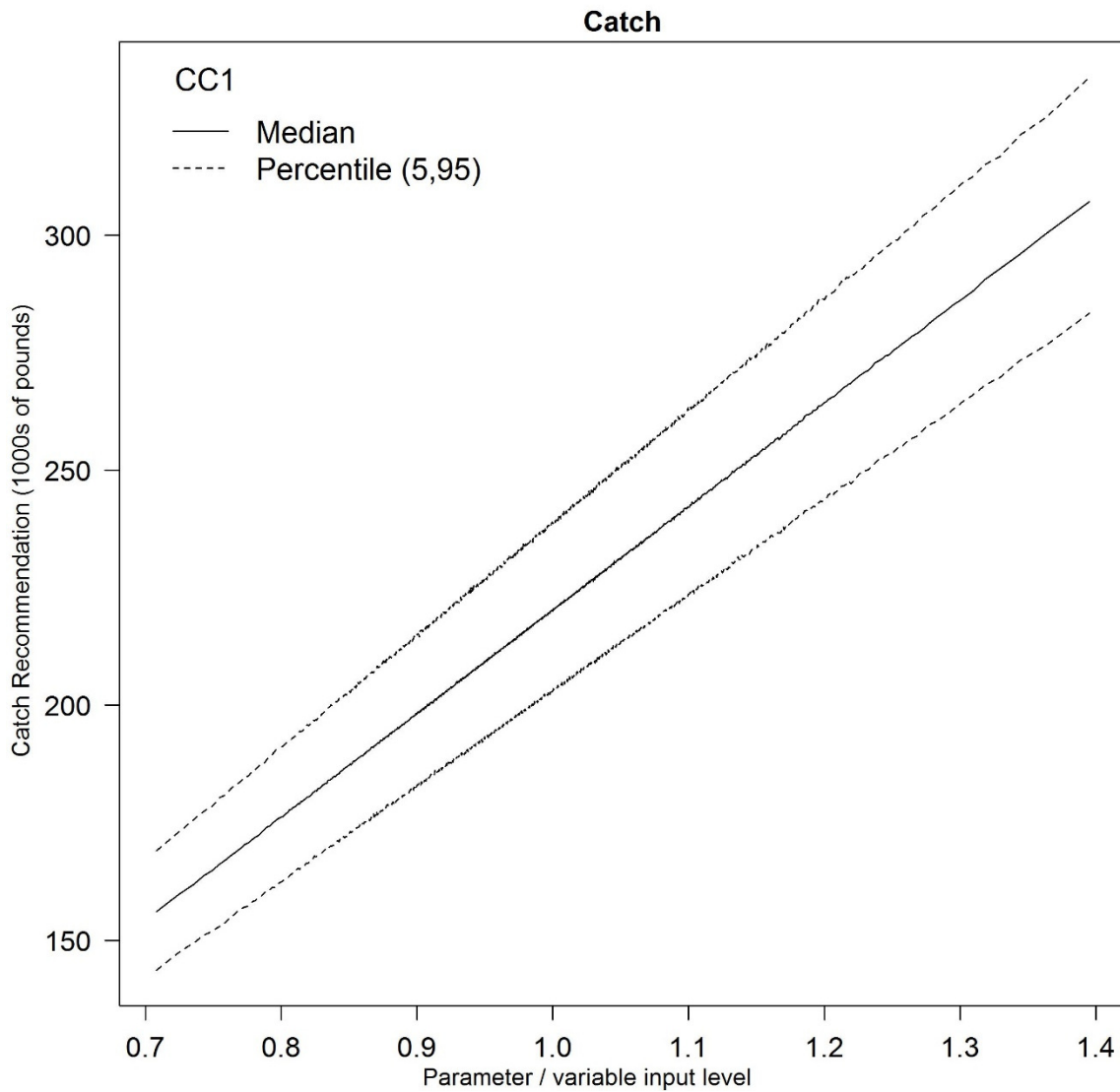
Figure 8.5 Sensitivity of the catch recommendation for Snowy Grouper to marginal changes in the required data inputs for CC1 (catch only). Note that ranges for parameter ranges are derived from the CV for each parameter.
