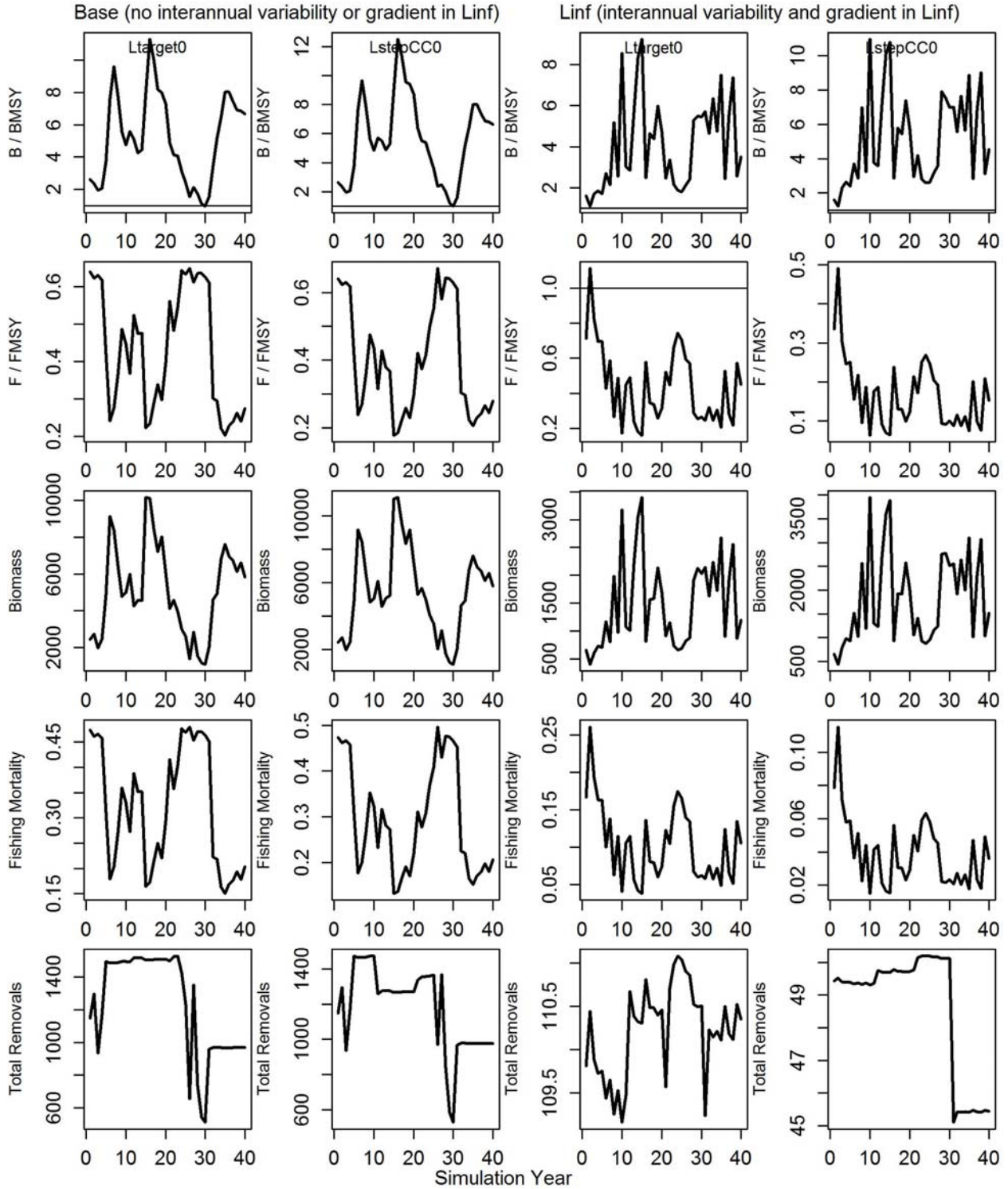
Figure 6.9 Comparison of stock status outputs and catches from the length-based methods for Wenchnan over the 40-year simulation period for a single simulation. Results are shown for the base model (no interannual variability of gradient in Linf) and a Linf sensitivity (15-20% interannual variability and a gradient of \pm 5\% in Linf). Outputs are as defined in Figure 6.2. Note that the y-axes differ between panels.
