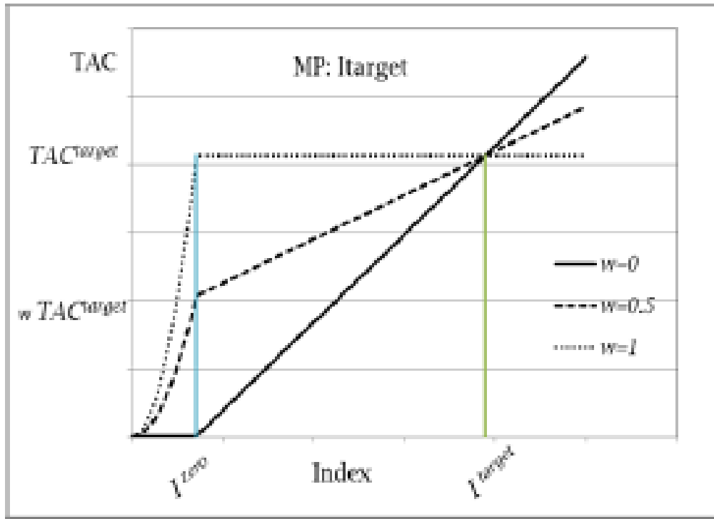
Figure 2 from Geromont and Butterworth (2014) supplementary material: Different forms of the Itarget0 method for three values of the control parameter w . Note that TAC is the terminology used for the catch recommendation in the source reference.
