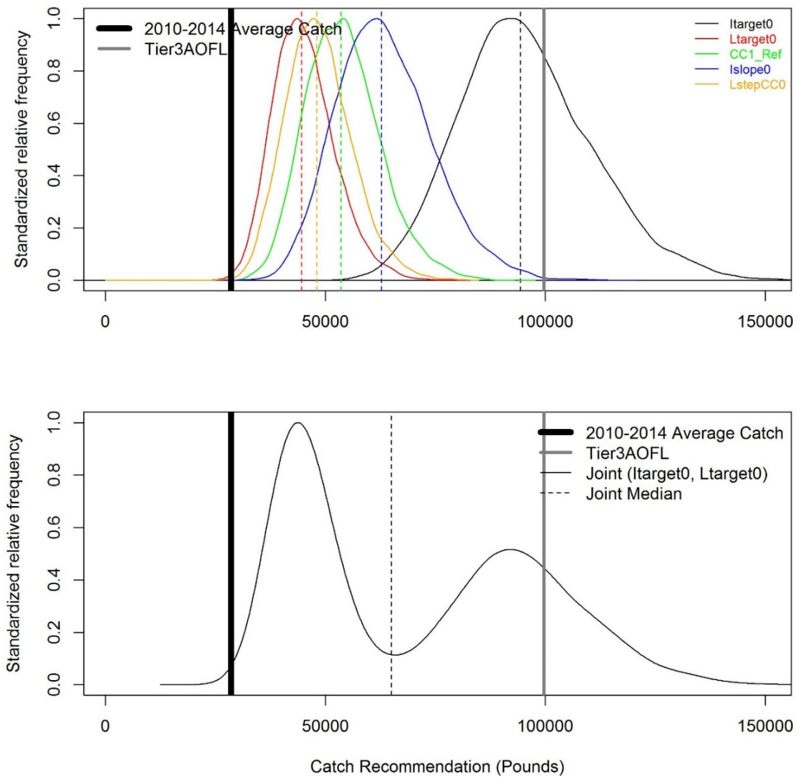
Figure 6.4 Distribution of the catch recommendation (in pounds) for Wenchman recommended by the five viable methods (top panel; dashed vertical lines identify medians) and a joint distribution assuming equal weighting of the top index-based ( I_{target0} ) and length-based ( L_{target0} ) methods according to performance in the MSE (bottom panel). The average catch between 2010 and 2014 (thick black line) and the OFL specified by the Tier3AStatusQuo (thick gray line) are included for comparison. The joint distribution (bottom panel) is recommended for providing management advice.
