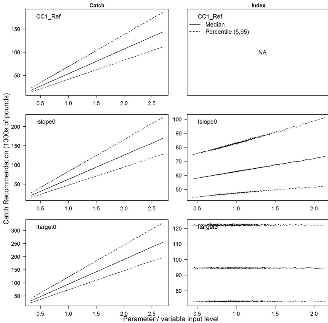
Figure 6.5 Sensitivity of the catch recommendation for Wenchman to marginal inputs in the required data inputs for CC1_Ref (catch only) and the index-based methods Islope0 and Itarget0 (Catch and index of abundance). Note that ranges for parameter ranges are derived from the CV for each parameter. NA indicates that the data input is not required. Sensitivity runs resulted in errors for both LstepCC0 and Ltarget0 and are therefore not shown.
