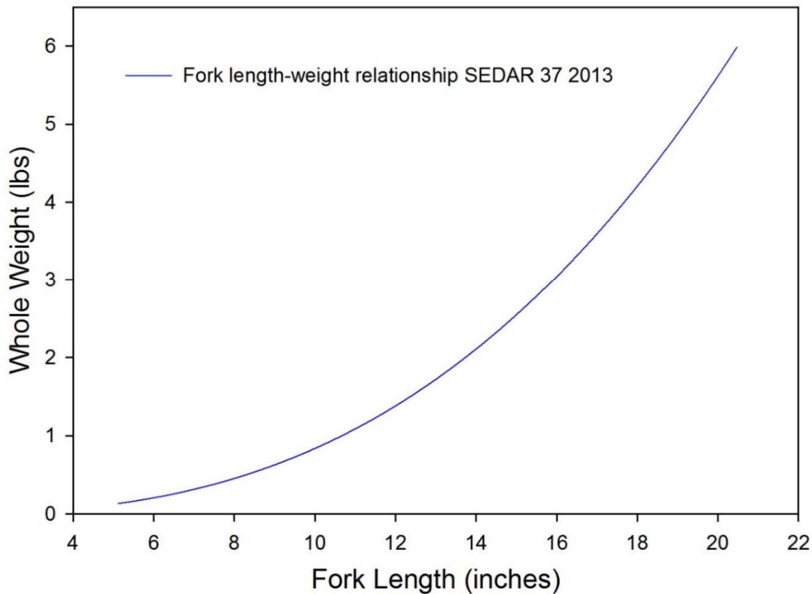
Figure 4.4.2.1. Hogfish length-weight relationship. Source: Conversion factors from SEDAR 37 (2014): \text{weight (g)} = 0.000095 * \text{FL(mm)}^2.74522 .
