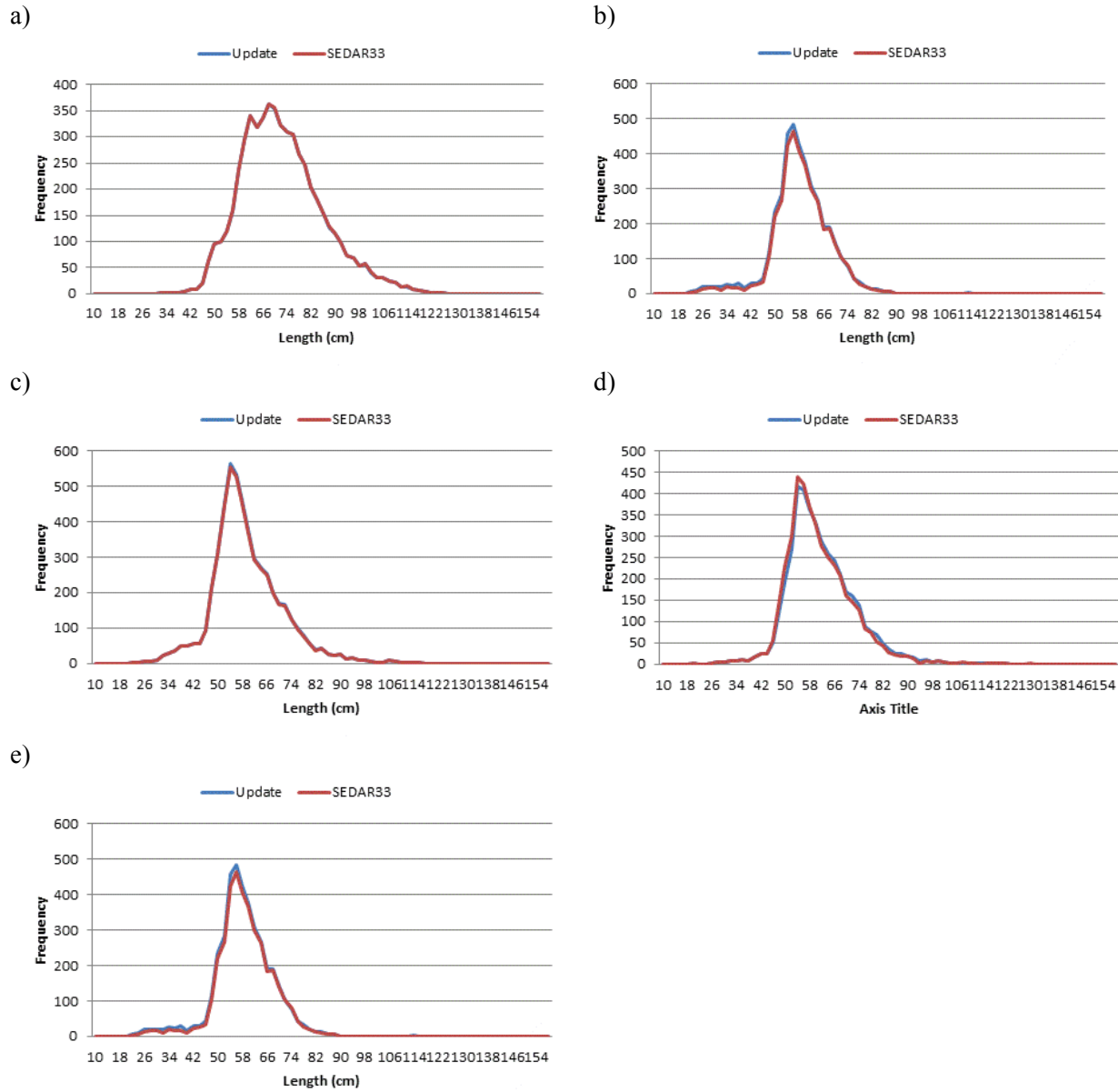
Figure 8. Length composition data of retained catch from the commercial a) vertical line and b) longline, and the recreational c) headboat, d) charter and e) private fleets. The figures do not include data from 2013-2015.
