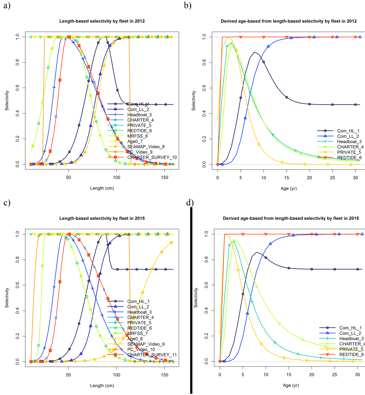
Figure 23. Length and age-based, fleet specific selectivity estimated from the a, b) SEDAR 33 and c, d) continuity models.
